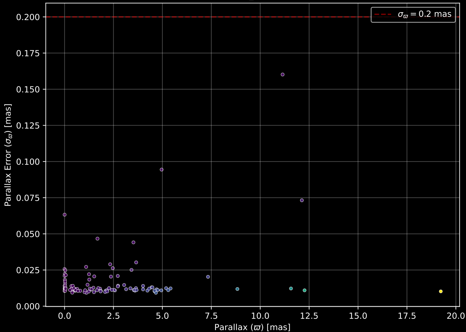
APOGEE DR17 Field: [276-32-O_TESS] Parallax Quality (n= 102)
