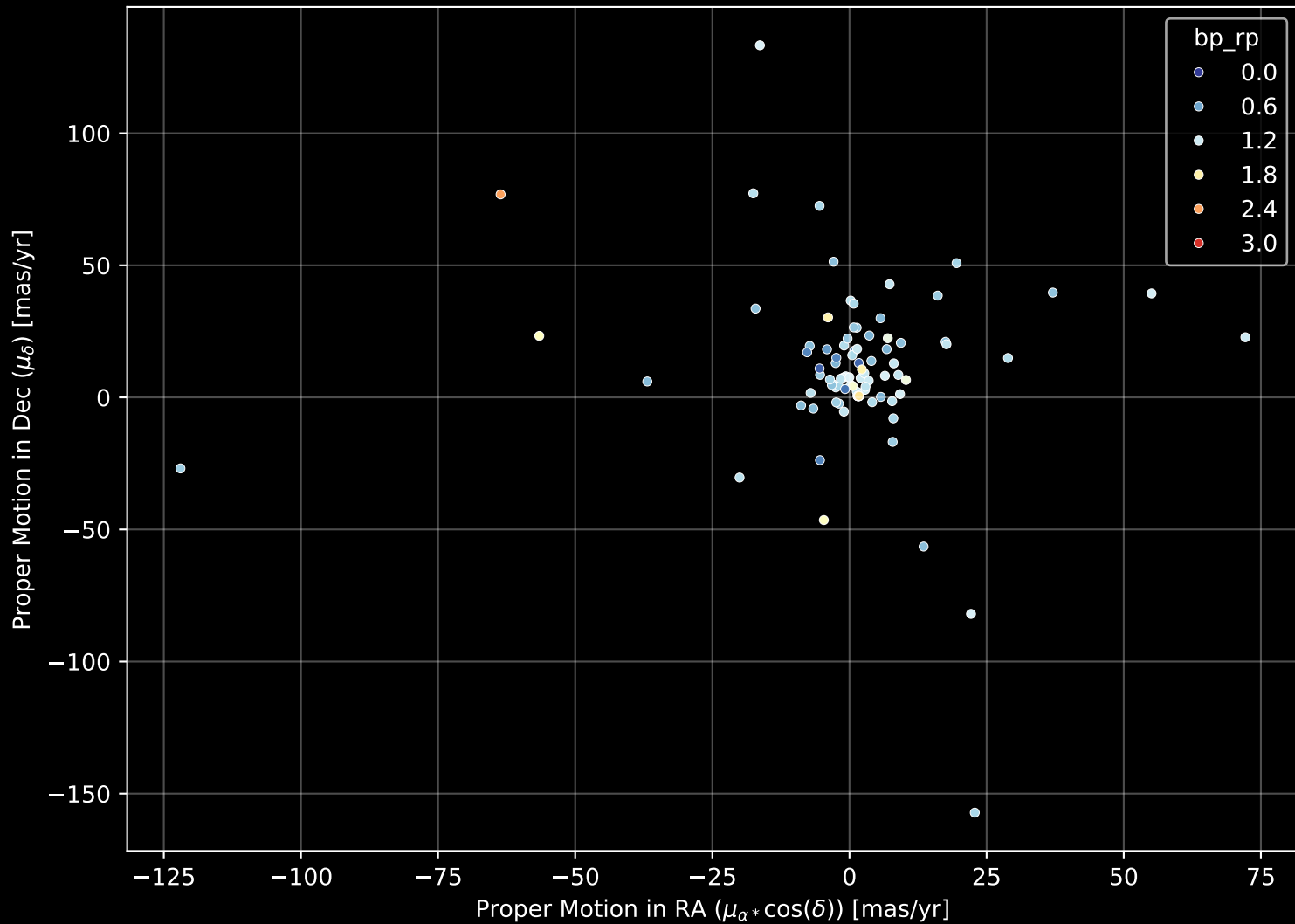
APOGEE DR17 Field: [276-32-O_TESS] Proper Motion Diagram (n= 102)
