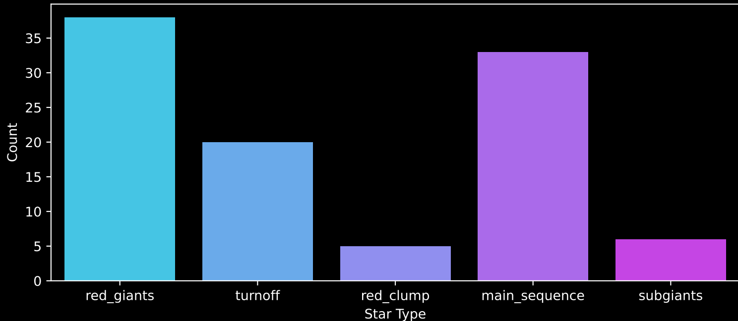
APOGEE DR17 Field: [276-32-O_TESS] Count plot of Star Type
