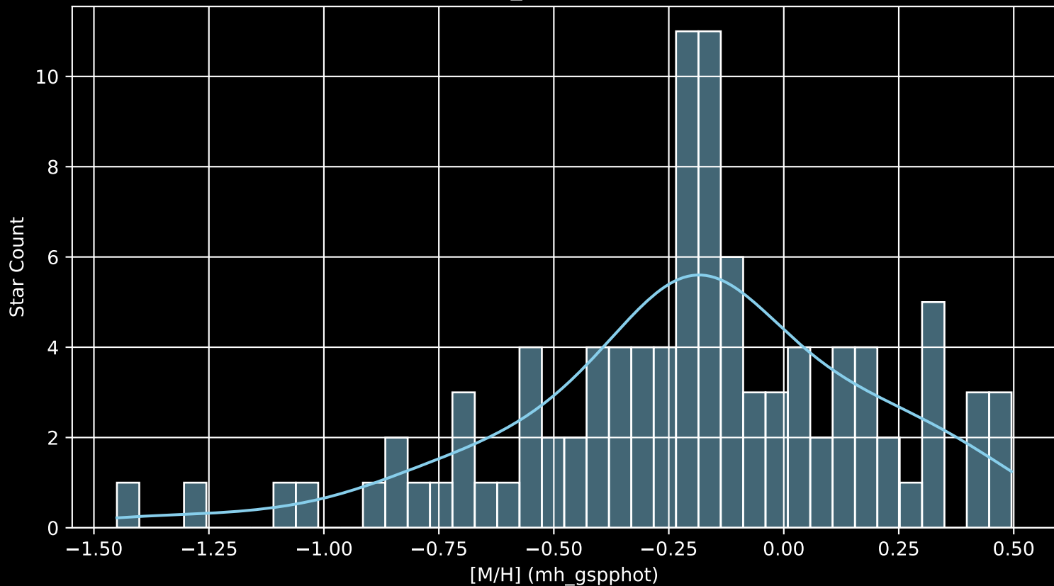
APOGEE DR17 Field: [276-32-O_TESS [M/H] (mh_gspphot) (n= 100)
