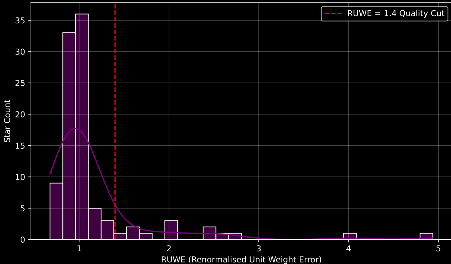
GAPOGEE DR17 Field [276-32-O_TESS] RUWE Distribution (n= 99)
